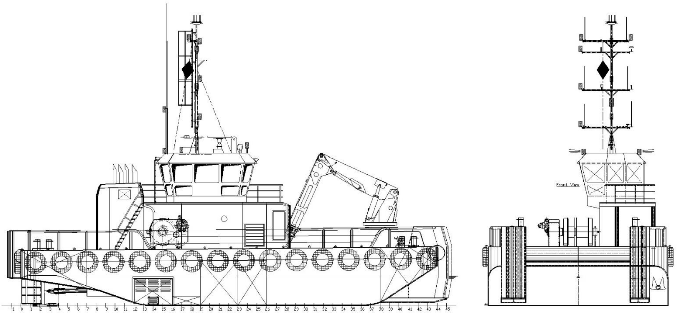
SIDE VIEW
